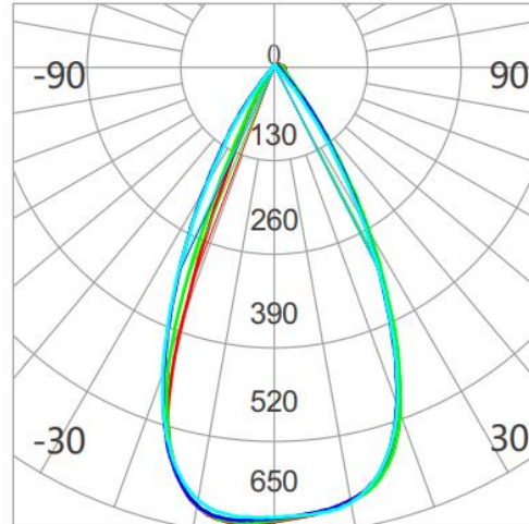
Average Beam Angle(50%): 50.7 DEG Beam Angle:51°
