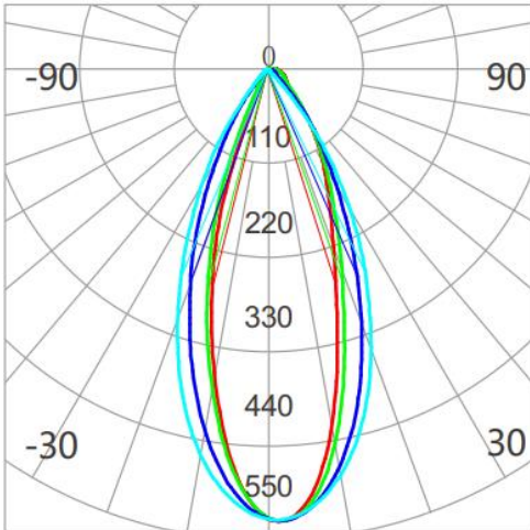
Average Beam Angle(50%): 39.7 DEG Beam Angle:32*50°
