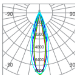
Average Beam Angle(50%): 25.5 DEG Beam angle:15°30° Efficacy:89.83lm/W
