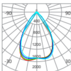
Average Beam Angle(50%): 68.1 DEG Beam angle:60° Efficacy:80.69lm/W
