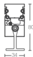
High-Profile Bracket
