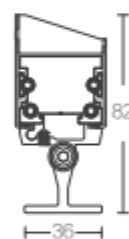
Adjustable bracket
