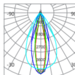
Average Beam Angle(50%): 32.2 DEG Beam angle:15°60° Efficacy:74.70lm/W
